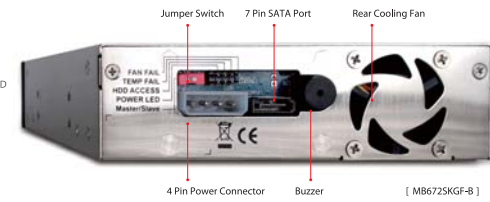
[ MB672SKGF-B ]
