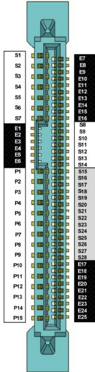
SFF-8639 U.2 pinout (Input)
