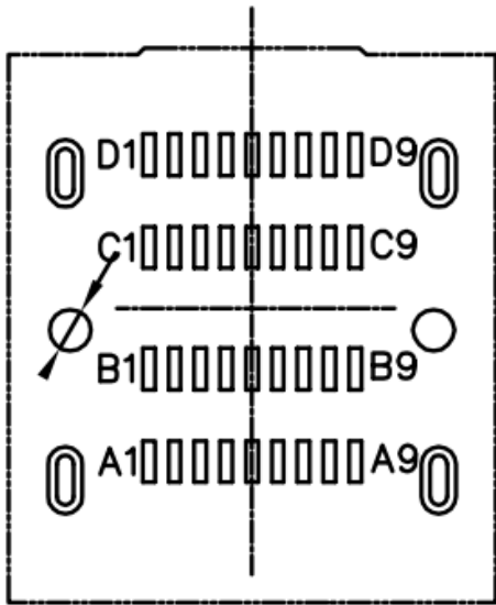
SFF-8643 miniSAS HD pinout (output)
