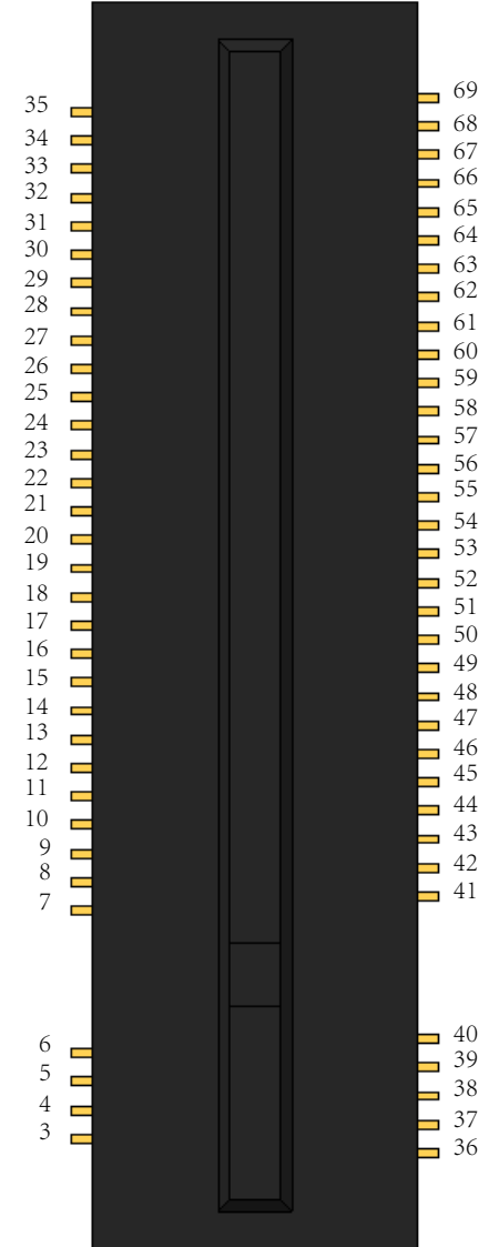
M.2 pinout (Input)
