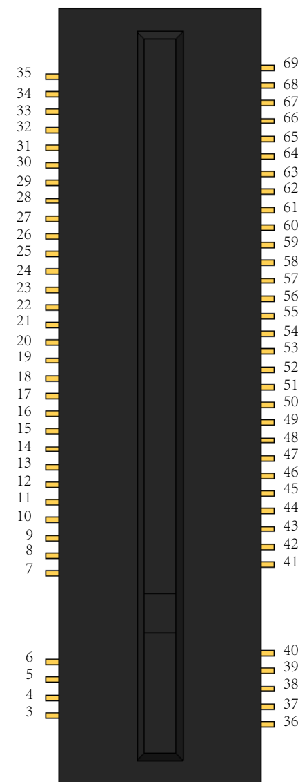
M.2 pinout (Input)
